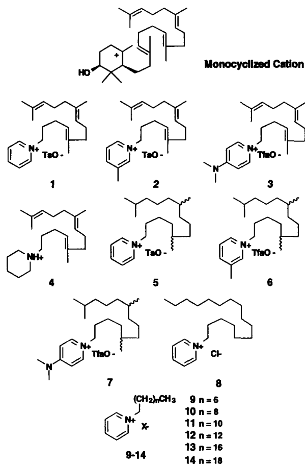
Figure 1. Compounds 1–14 which mimic a monocyclized cationic species (transition state or high-energy intermediate). TsO − : p -Toluenesulfonate; TfaO − : Trifluoroacetate.
