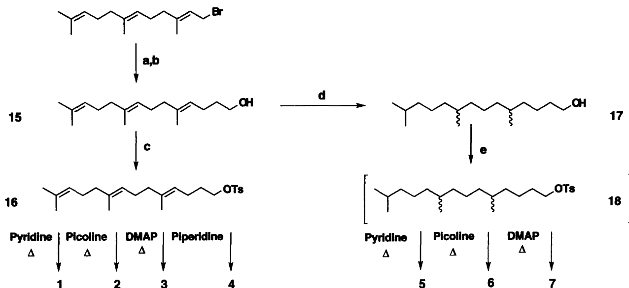
Scheme 2. Synthesis of compounds 1–7. (a) C 2 H 5 O 2 CCH 2 Cu(I), THF, −30 °C; (b) LiAlH 4 , Et 2 O; (c) TsCl, Et 3 N, CH 2 Cl 2 ; (d) H 2 , Pd/C; (e) TsCl with the pyridine derivatives as solvent.
